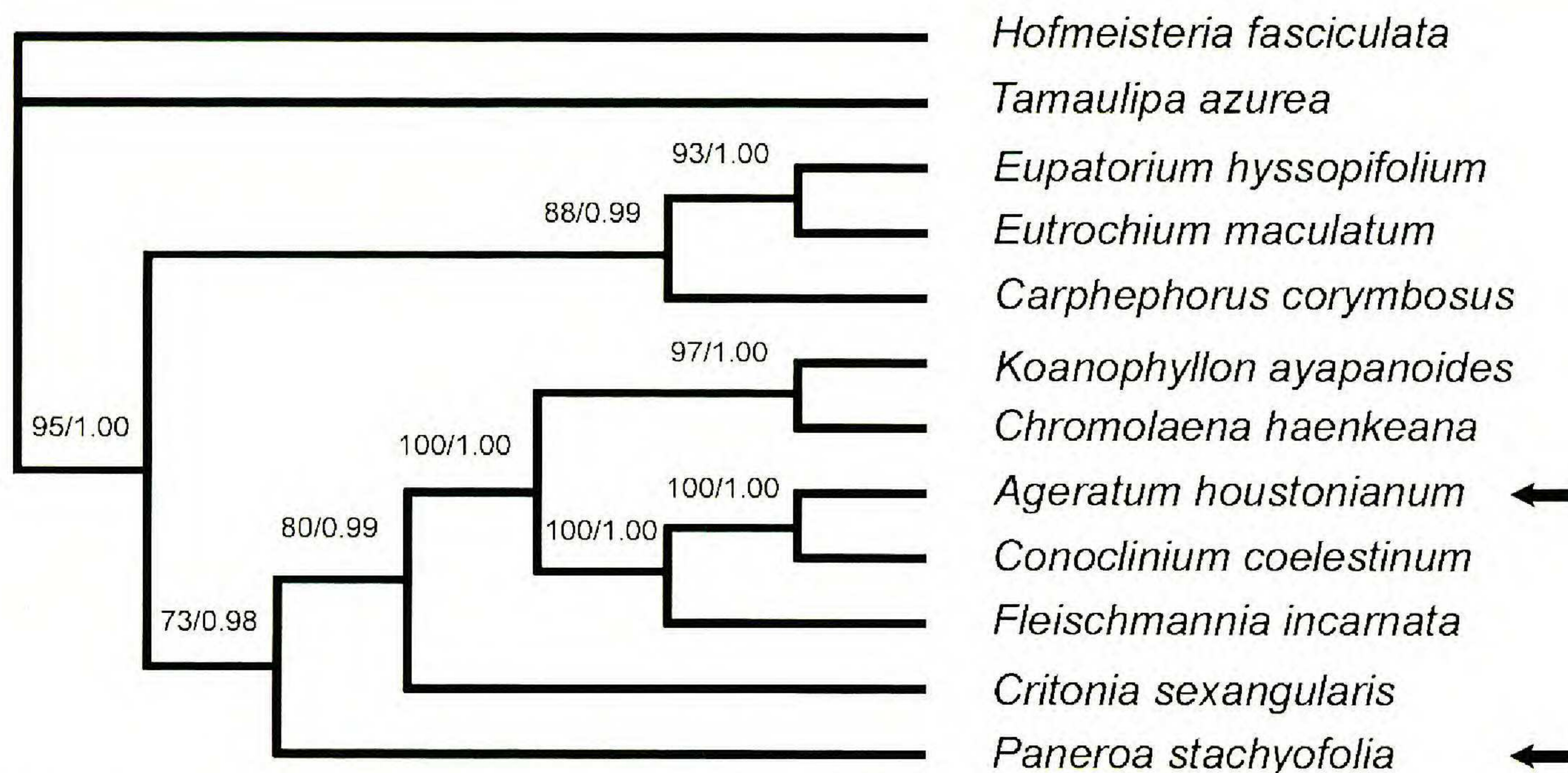
Figure 2. Single most parsimonious tree (length = 346 steps; consistency index [CI] = 0.91; retention index [RI] = 0.78) from analysis of chloroplast DNA data (total of 4200 aligned base pairs) for Paneroa and related genera, with bootstrap support (1000 replicates)/Bayesian posterior probabilities shown above branches, showing the placement of Paneroa relatively distant from Ageratum (arrows). Voucher data for chloroplast DNA sequence data used to prepare the tree are provided in Appendix 1.
